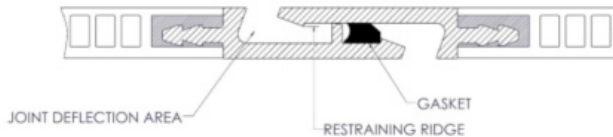
VYLON SLIPLINER ANTI-DISENGAGING COUPLER
